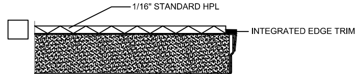
CORNER SECTION - 1/16" HPL WITH INTEGRATED TRIM
