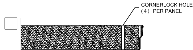
CORNER SECTION - BARE CORNERLOCK
