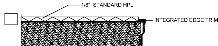
CORNER SECTION - 1/8" HPL WITH INTEGRATED TRIM
